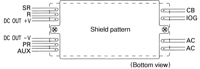
Fig.5.2 Shield pattern lay out
