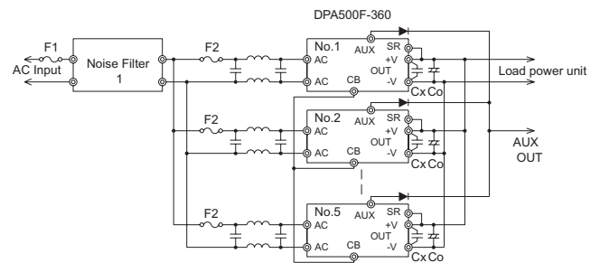
Fig.4.1 Connection for parallel operation
