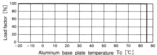
Fig.5.3 Derating curve
