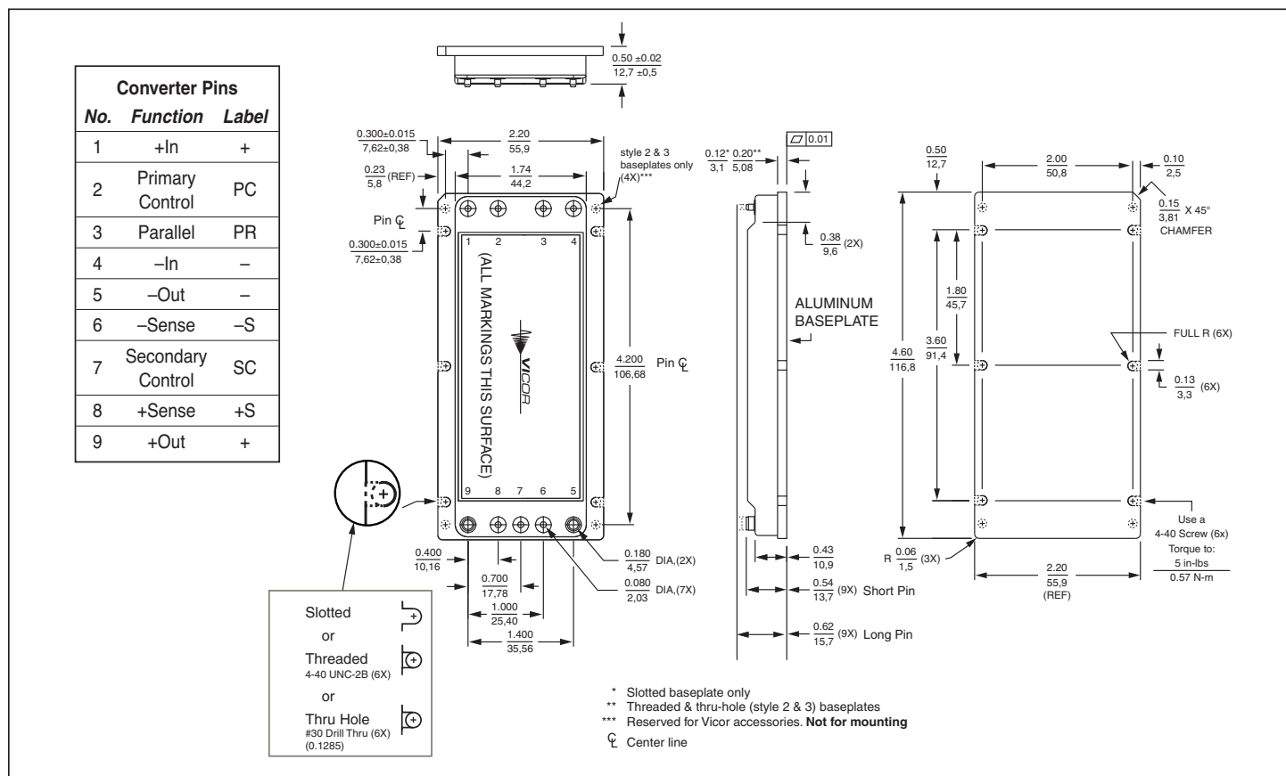
Figure 13 — Module outline
