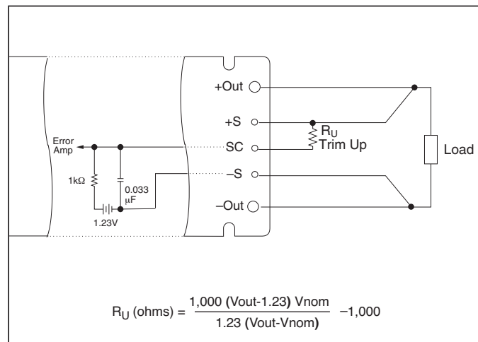
Figure 8 — Output voltage trim up circuit.
