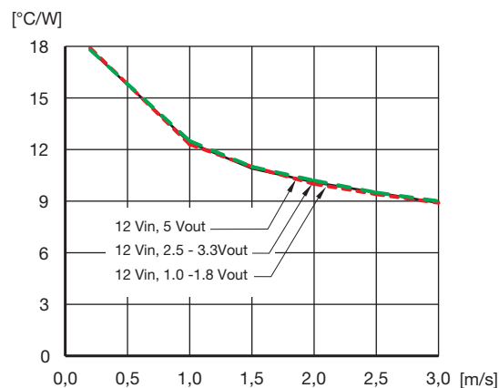
Thermal resistance vs. airspeed measured at the regulator.
