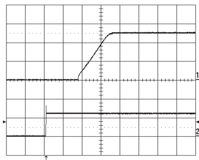
Start-up at I_O = 10\text{ A} resistive load at T_{ref} = +25\text{ }^{\circ}\text{C} , V_{in} = 12\text{ V} . Start enabled by connecting V_{in} . Top trace: output voltage (2 V/div.). Bottom trace: input voltage (10 V/div.). Time scale: 2 ms/div.
