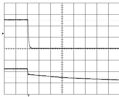
Turn-off at I_O = 10\text{ A} resistive load at T_{ref} = +25\text{ }^{\circ}\text{C} , V_{in} = 12\text{ V} . Turn-off enabled by disconnecting V_{in} . Top trace: output voltage (2 V/div.). Bottom trace: input voltage (10 V/div.). Time scale: 2 ms/div.
