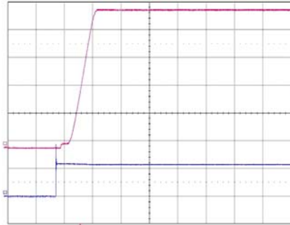
Start-up enabled by connecting V_i at: T_{ref} = +25^\circ\text{C} , V_i = 12\text{ V} , I_o = 16\text{ A} resistive load. Top trace: output voltage (1 V/div.). Bottom trace: input voltage (10 V/div.). Time scale: (5 ms/div.).
