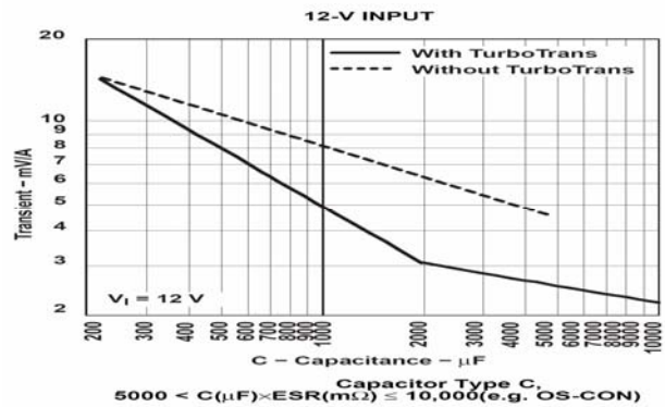
Type C TurboTrans C_o Values and Required R_{TT} Selection Table
