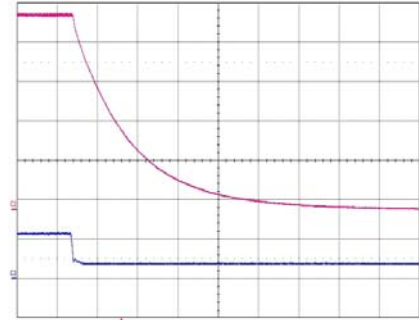
Shut-down enabled by disconnecting V_i at: T_{ref} = +25^\circ\text{C} , V_i = 12\text{ V} , I_o = 16\text{ A} resistive load. Top trace: output voltage (1 V/div.). Bottom trace: input voltage (10 V/div.). Time scale: (0.5 ms/div.).
