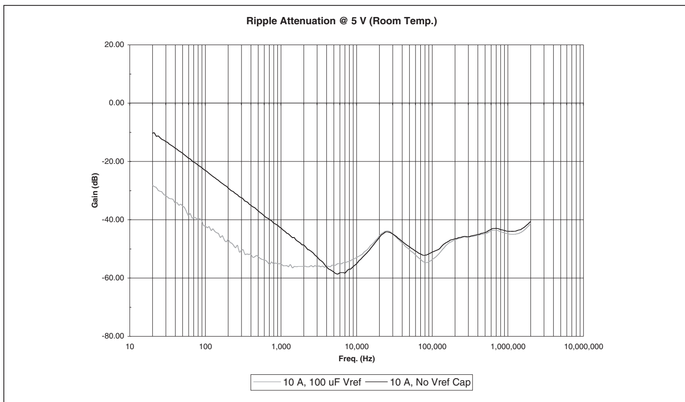
Figure 3a, 3b —Curves demonstrating the small signal attenuation performance as measured on a network analyzer with a typical module at (a) 28 V and 10 A output and (b) 5 V and 10 A. The low frequency attenuation can be enhanced by connecting a 100 \mu F capacitor, CHR, to the VREF pin as shown in Figures 1 and 2.
