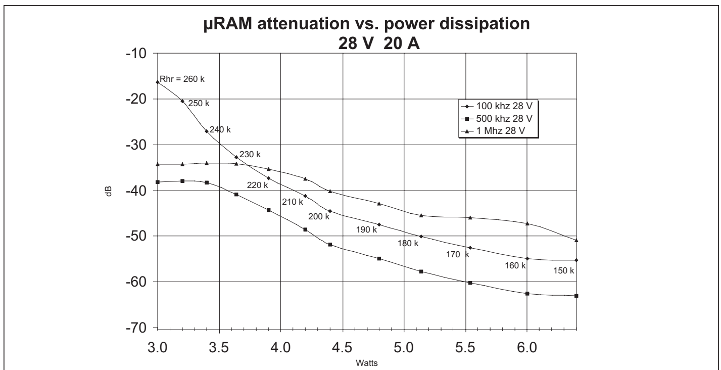
Figure 4c – 4d —MicroRam attenuation vs. power dissipation at 3 V 20 A, and 28 V 20 A.
