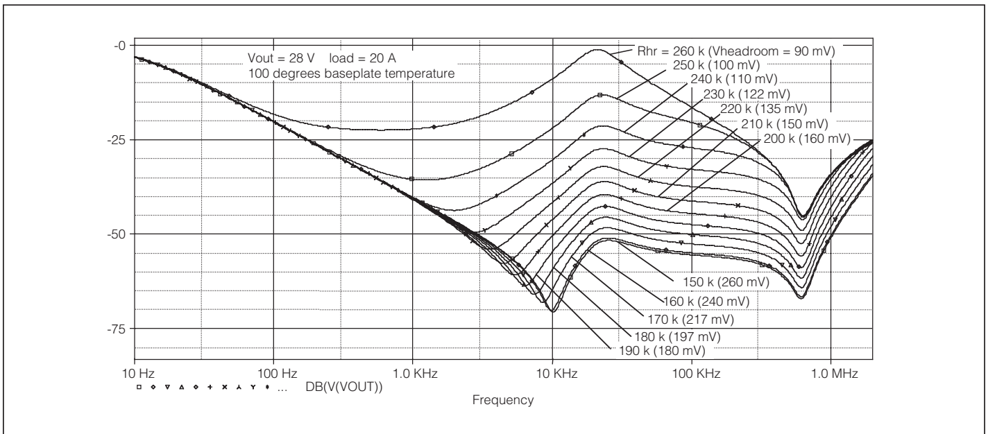
Figure 4a — 4b — Simulated graphs demonstrating the tradeoff of attenuation versus headroom setting at 20 Amps and an equivalent 100°C baseplate temperature at 3 V and 28 V.
