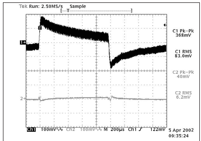
Figure 10 — V375A28C600B and \mu RAM; Input and output dynamic response C TRAN = 820 \mu F Electrolytic; 32.5% of load step of 6.5 A (10 A – 16.5 A); RHR = 178 k (Configured as in Figs. 1 & 2)
