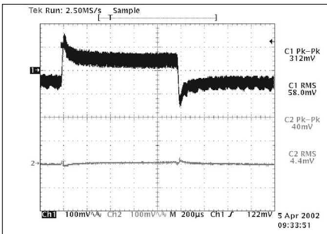
Figure 9 — V375A28C600B and \mu RAM; Input and output dynamic response no added C TRAN ; 20% of 20 A rating load step of 4 A (10 A – 14 A); RHR = 178 k (Configured as in Figs. 1 & 2)
