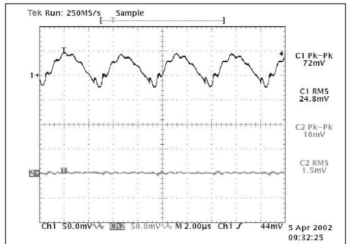
Figure 8 — V375A28C600B and \mu RAM; Input and output ripple @50% (10 A) load CH1 = Vi; CH2 = Vo; Vi-Vo = 332 mV; RHR = 178 k
