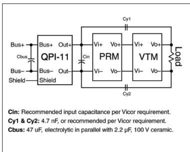
Figure 2 – QPI-11 Typical application schematic
