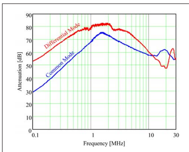
Figure 3 – QPI-11 network analyzer attenuation curves
