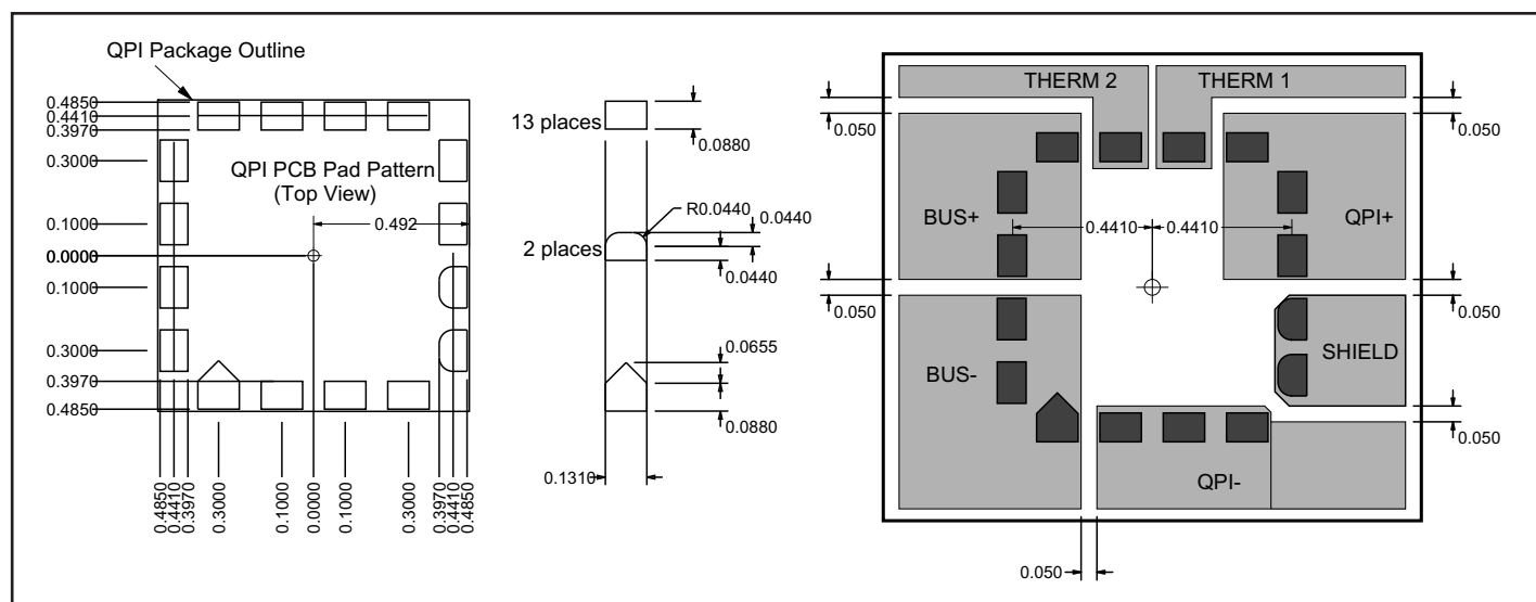
Figure 12 – Recommended PCB solder mask dimensions and layout. Use 1.3mm clearance around shield pads 5 & 6 to adjacent lands. See Figures 9 & 10 for recommended connection layouts.
