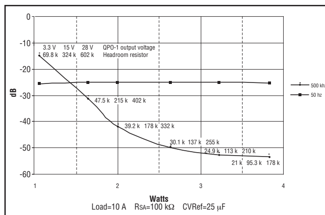
Figure 9 - Attenuation vs. power dissipation without slope adjust.
