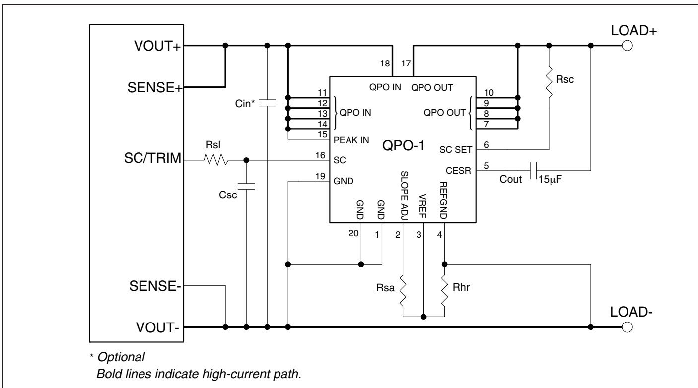
Figure 4 – Simplest application of QPO-1 when the SC/Trim pin is available, see text.
