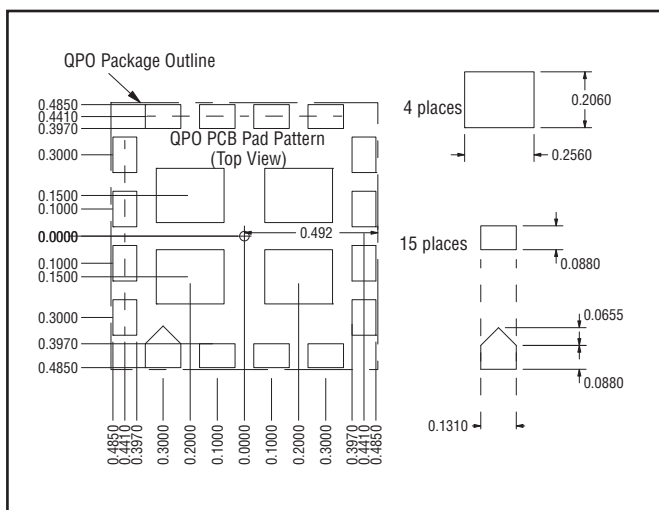
Figure 14 - LAND GRID ARRAY PCB Solder Mask Openings (dimensions in inches)
