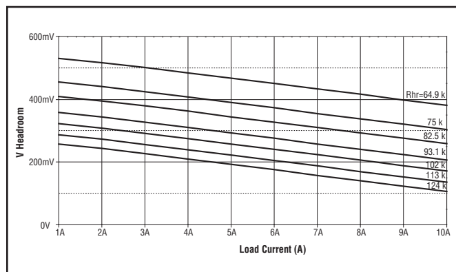
Figure 8 - Effect of slope adjust on headroom value with increasing current and RSA = 8.2 k.
