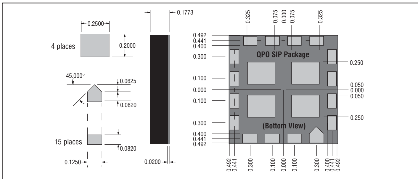
Figure 13 - Package dimension drawing (dimensions in inches)
