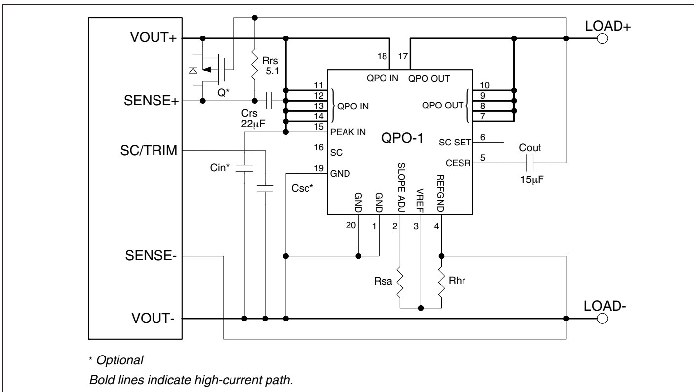
Figure 3 – Use this circuit for applications requiring remote sensing. Components marked * are optional, see text.
