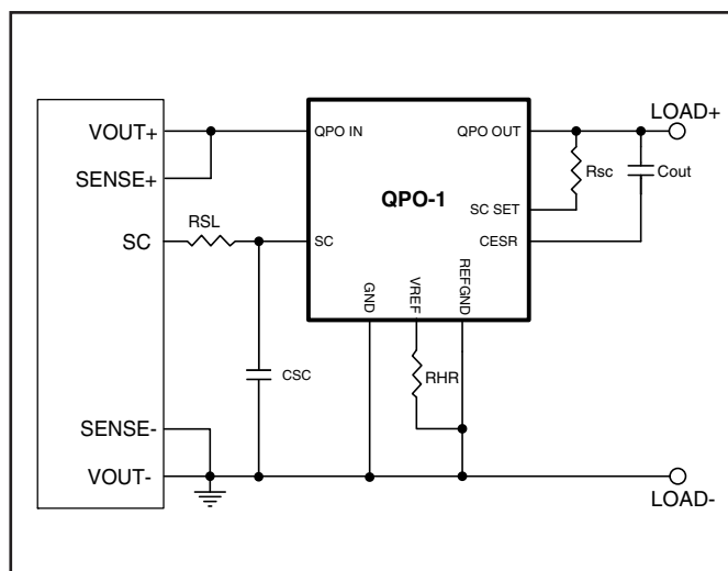
Figure 1 – Typical Application: SC/Trim supports applications that don't require remote sense.
