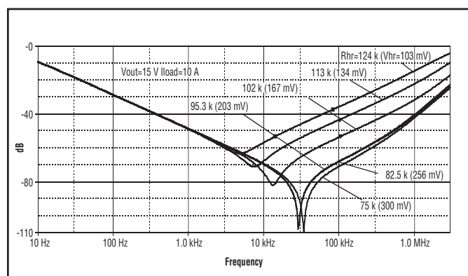
Figure 7 – Attenuation at different headroom settings with 25 \mu F capacitor connected to V_{ref} .
