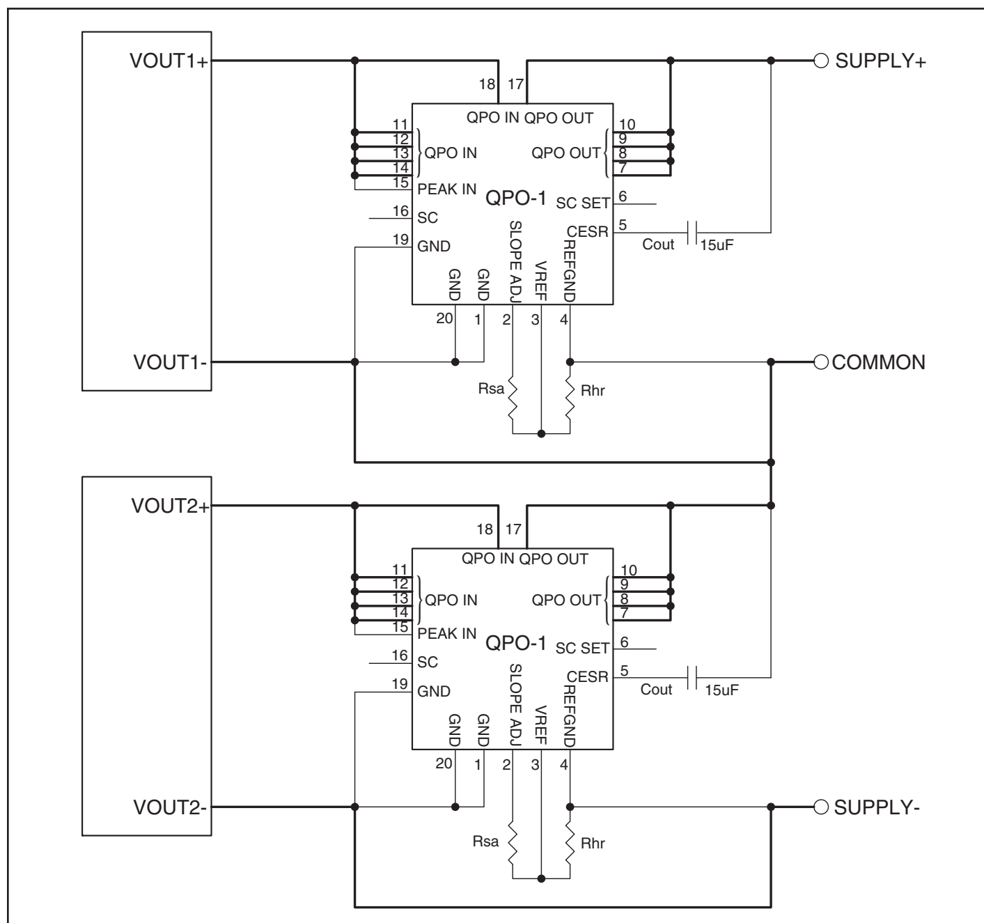
Figure 12- Schematic for +/- supply application. Circuit shown is for an open loop configuration. See text and schematic showing SC/Trim and remote sense application if required. Dark lines show high-current path.
