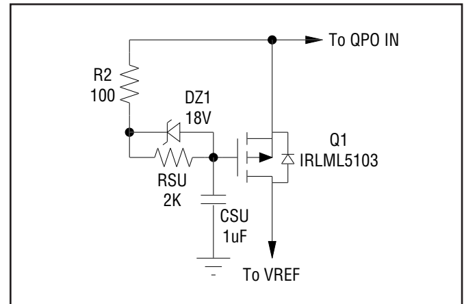
Figure 11 - Zero Headroom Start-up Circuit.
