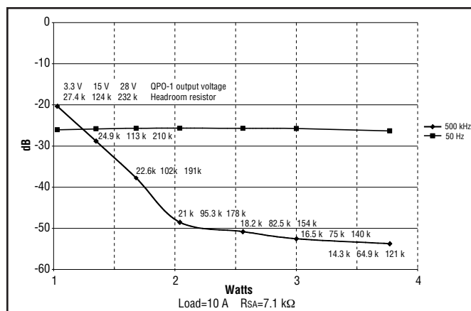
Figure 10 - Attenuation vs. power dissipation with slope adjust.
