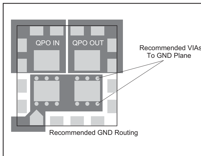
Figure 15 - Recommended copper pattern for LGA mounting showing QPO pads and minimum copper landing. Pattern should be on 2 oz. copper with vias, placed outside of device pad solder mask openings, used to connect to internal layers (if required).
