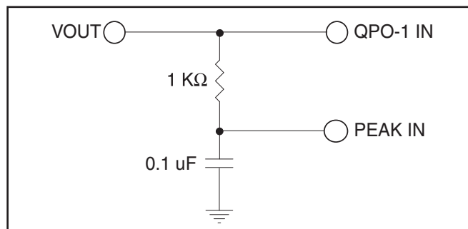
Figure 5 – Peak detect disable circuit.
