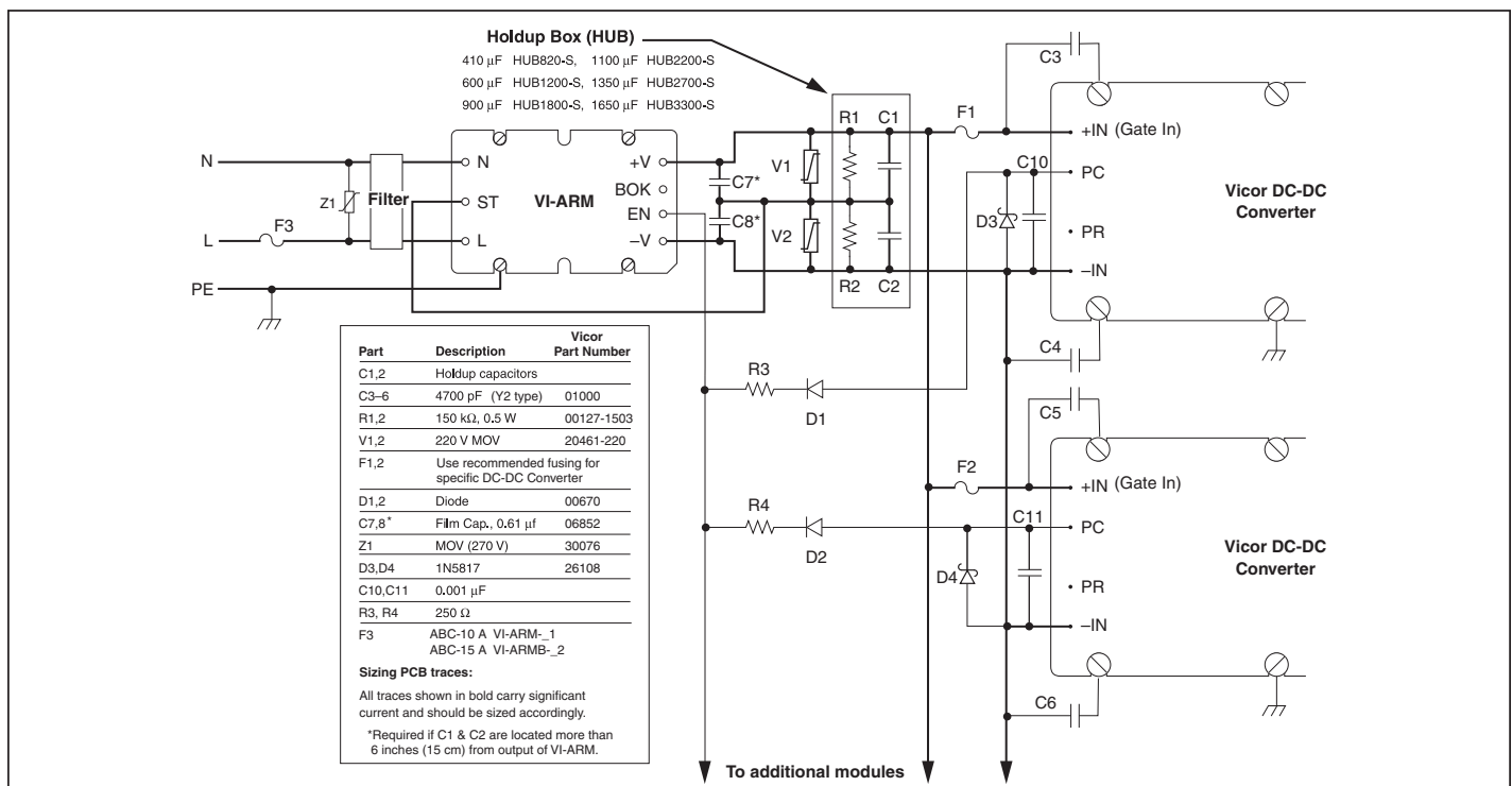
Figure 10 — Converter connections
