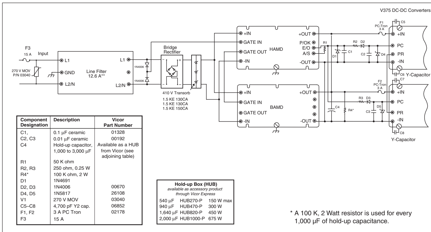
Figure 5 — Connection Diagram, HAMD / BAMD / V375 DC-DC Converters
