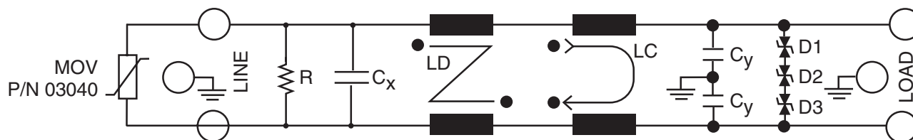
C_x = 1.5 \text{ uF}(x2)SH C_y = .01 \text{ uF} SH LC = 6.9mH LD = .72mH R = 235K OHM D1,2 = 1.5KE130CA D3 = 1.5KE150CA
