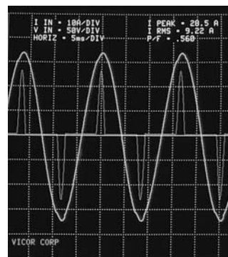
Figure 2a – Without PFC
