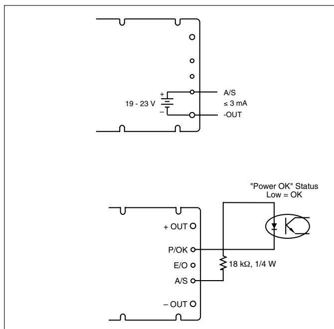
Figure 6 — Auxiliary Supply (A/S)
