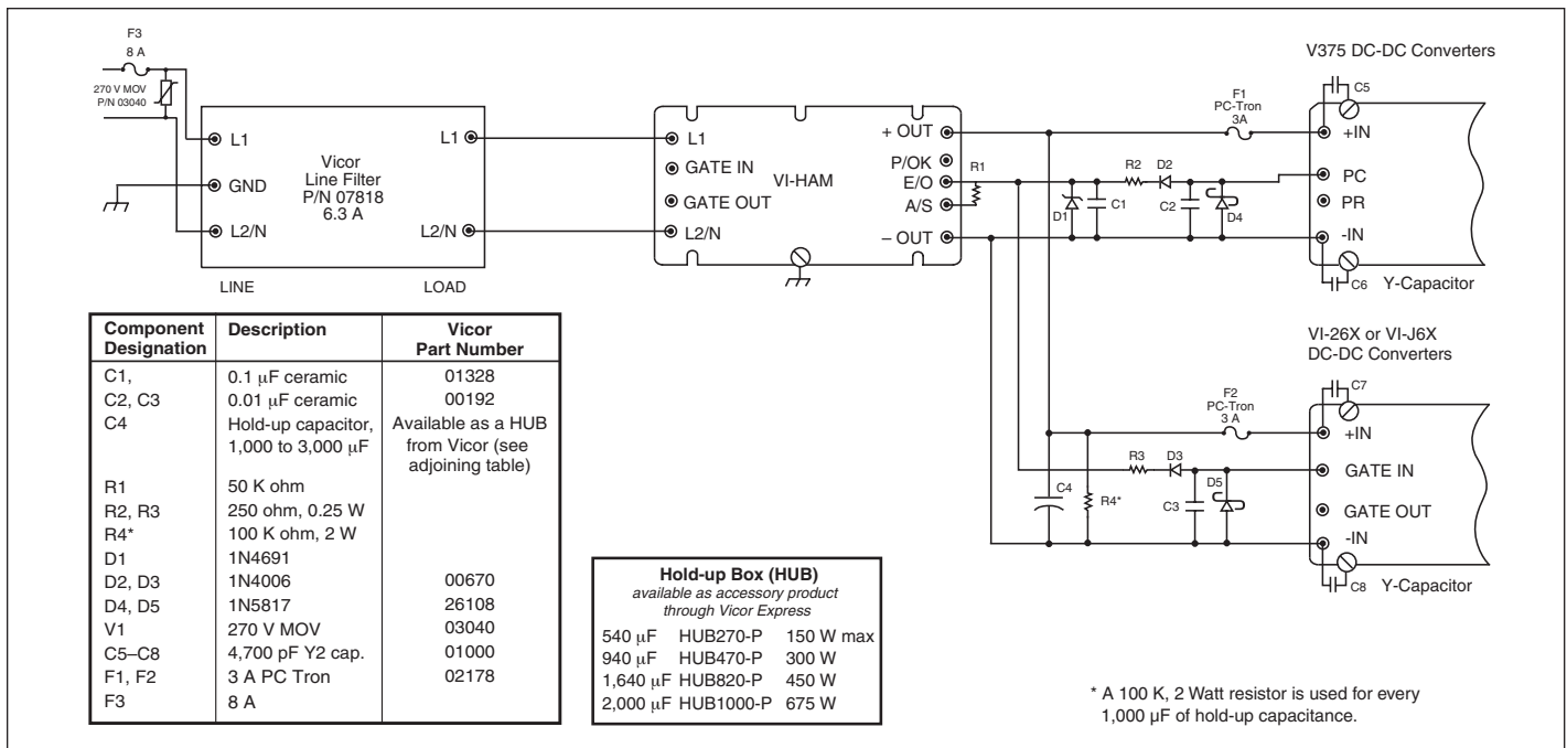
Figure 4 — Connection diagram HAM / DC-DC converters
