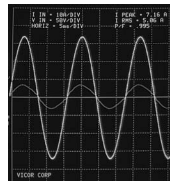
Figure 2b – With PFC
