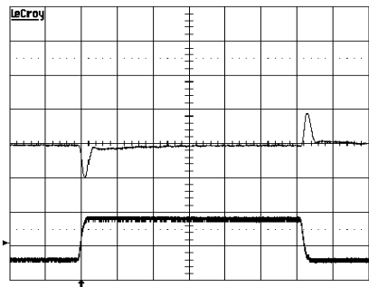
Output voltage response to load current step- change (3-9-3 A) at: T_{ref} = +25^{\circ}\text{C} , V_i = 53\text{ V} . Top trace: output voltage (500mV/div.). Bottom trace: load current (5 A/div.). Time scale: (0.1 ms/div.).
