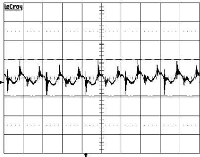
Output voltage ripple at: T_{ref} = +25^{\circ}\text{C} , V_i = 53\text{ V} , I_o = 12\text{ A} resistive load. Trace: output voltage (20mV/div.). Time scale: (2 μs/div.).
