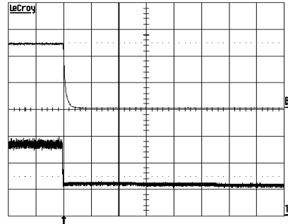
Shut-down enabled by disconnecting V_i at: T_{ref} = +25^{\circ}\text{C} , V_i = 53\text{ V} , I_o = 12\text{ A} resistive load. Top trace: output voltage (5 V/div.). Bottom trace: input voltage (20 V/div.). Time scale: (1 ms/div.).
