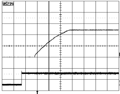
Start-up enabled by connecting V_i at: T_{ref} = +25^{\circ}\text{C} , V_i = 53\text{ V} , I_o = 12\text{ A} resistive load. Top trace: output voltage (5 V/div.). Bottom trace: input voltage (50 V/div.). Time scale: (5 ms/div.).
