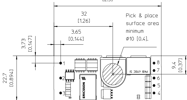
RECOMMENDED FOOTPRINT
