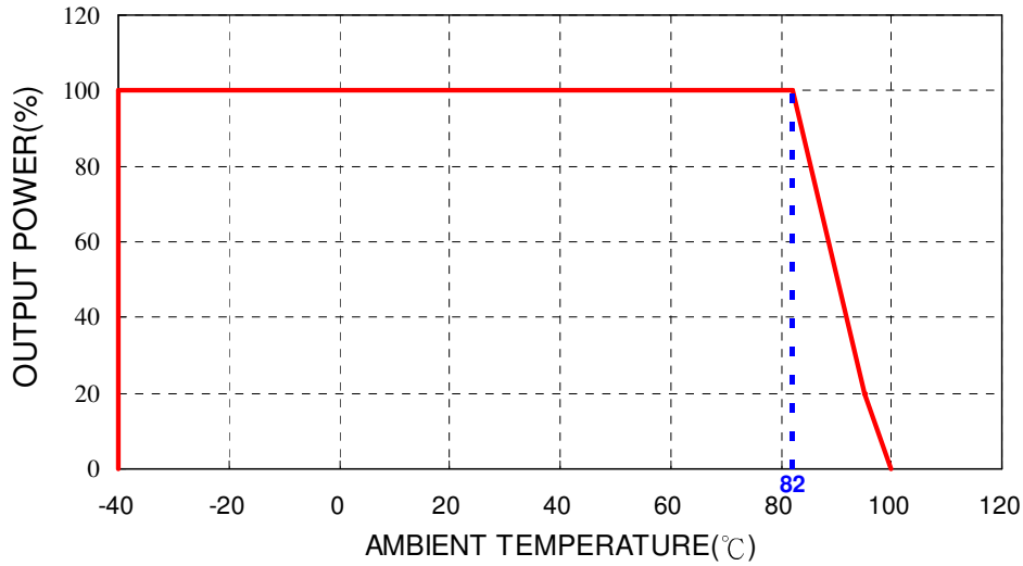
PM-10MD091 Derating curve
