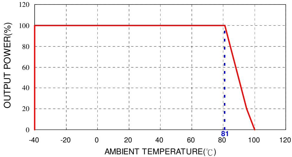
PM-11MD092 Derating curve
