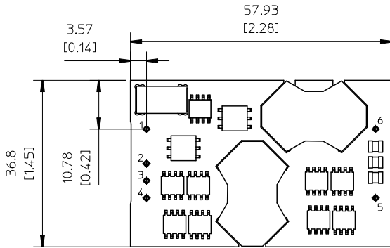
RECOMMENDED FOOTPRINT TOP VIEW
