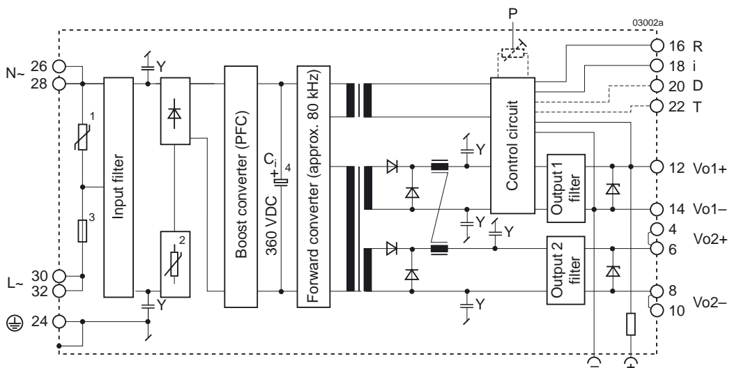
Fig. 2 Block diagram of double-output models
