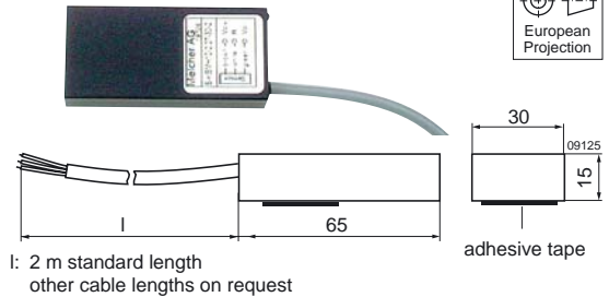
Battery temperature sensor
