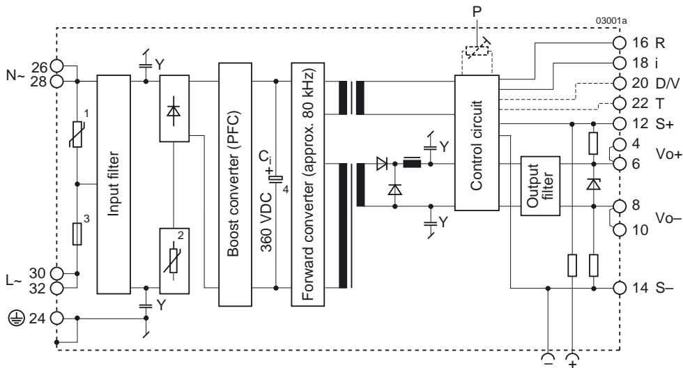
Fig. 1 Block diagram of single-output converters
