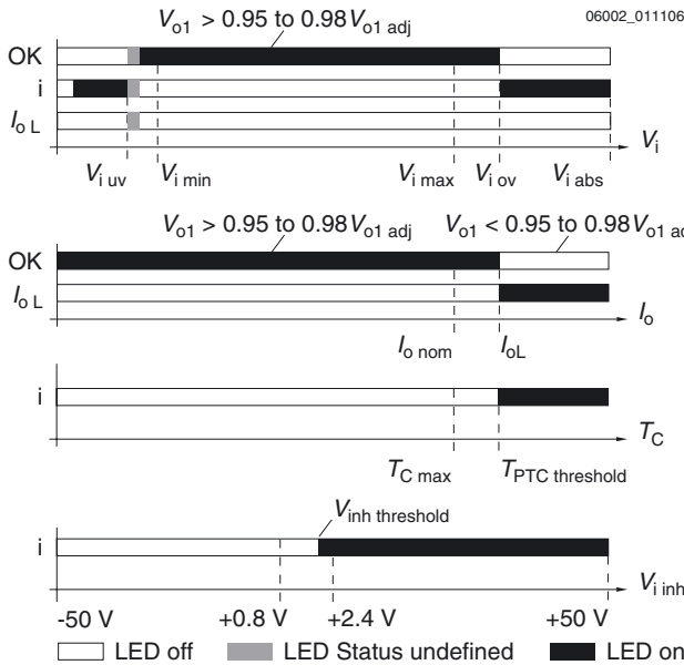
Fig. 23 LED indicators
