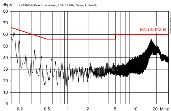
Fig. 26 Conducted emissions (peak) at the phase input according to EN 55011/22, measured at V_{in, nom} and I_{o, nom} (LKP5660-6R). The neutral line performs quite similar.
