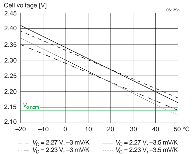
Fig. 25 Trickle charge voltage versus temperature for defined temperature coefficient. V_{o\text{ nom}} is the output voltage with open R-input.
