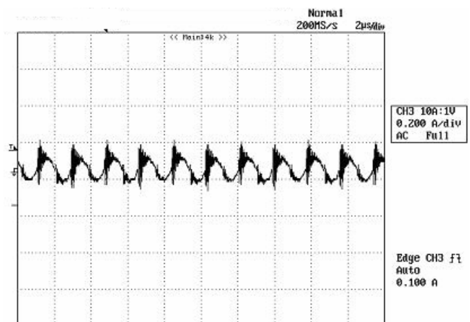
Figure 11: Input Terminal Ripple Current, i_c , at full rated output current and nominal input voltage with 12\mu H source impedance and 33\mu F electrolytic capacitor (200 mA/div, 2µs/div).
