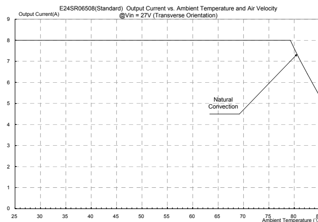
Figure 22: Output current vs. ambient temperature and air velocity @ V_{in}=27V (Transverse Orientation)
