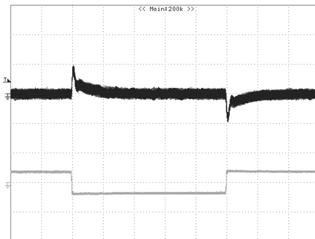
Figure 9: Output voltage response to step-change in load current (75%-50%-75% of I_o , max; di/dt = 2.5A/\mu s ). Load cap: 330\mu F , 35m\Omega ESR solid electrolytic capacitor and 1\mu F ceramic capacitor. Top Trace: V_{out} (100mV/div, 200us/div), Bottom Trace: I_{out} (5A/div). Scope measurement should be made using a BNC cable (length shorter than 20 inches). Position the load between 51 mm to 76 mm (2 inches to 3 inches) from the module
