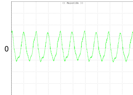
Figure 11: Input Terminal Ripple Current, i_c , at full rated output current and nominal input voltage with 12 \mu H source impedance and 100 \mu F electrolytic capacitor (100 mA/div, 2 \mu s/div)
