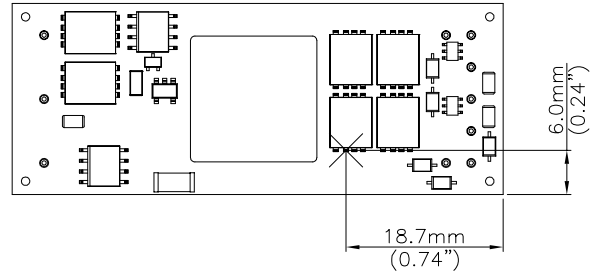
Figure 20: Temperature measurement location The allowed maximum hot spot temperature is defined at 117 °C.
