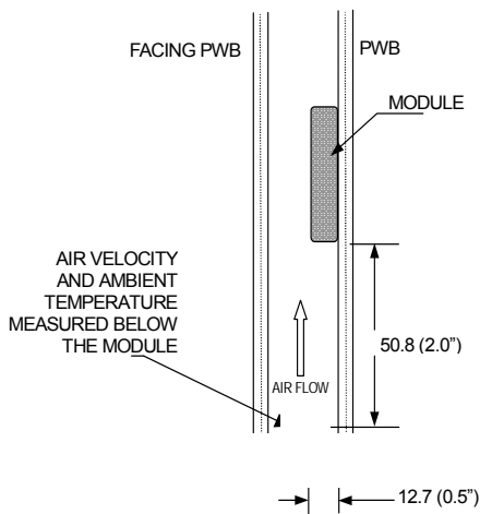
Figure 19: Wind tunnel test setup
