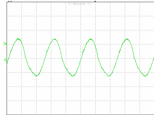
Figure 11: Input Terminal Ripple Current, i_c , at full rated output current and nominal input voltage with 12 \mu\text{H} source impedance and 33 \mu\text{F} electrolytic capacitor (200 mA/div, 1 \mu\text{s} /div)
