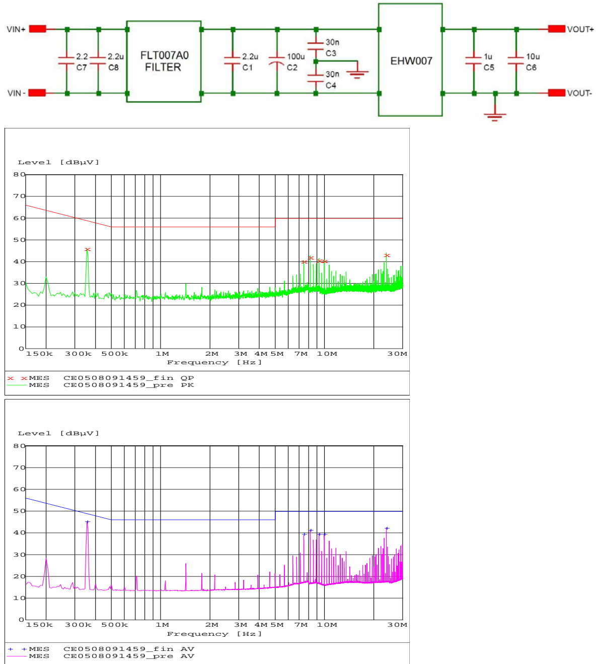
Figure 21. EMC Considerations
