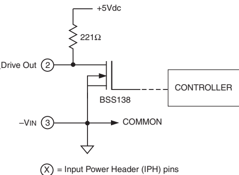
Typical Power Good External LED Lamp Wiring
