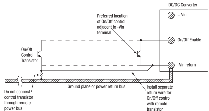
Figure 8. On/Off Enable Control Ground Bounce Protection
