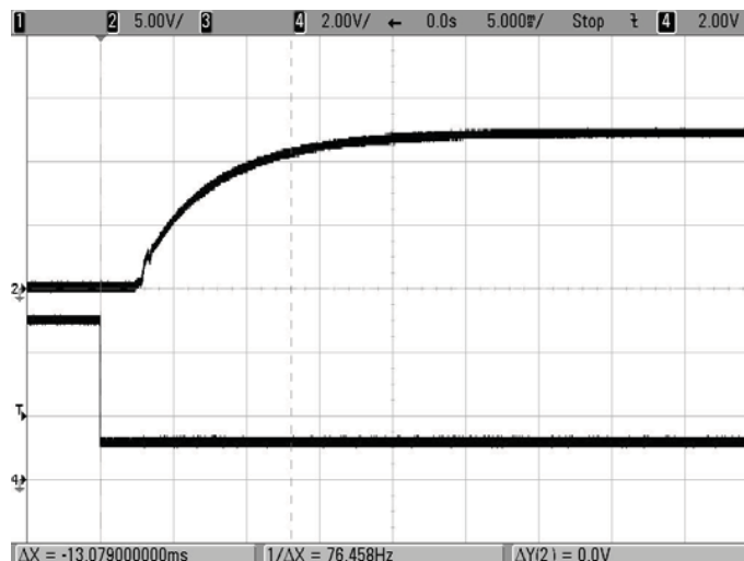
Enable Start-up (Vin=48V, Iout=5A, Load=1000µF Ta=+25°C) Trace 2=Output, Trace 4= Enable.
