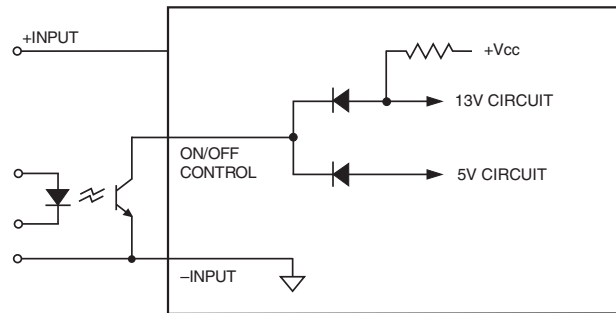
Figure 5. Driving the Negative Polarity On/Off Control Pin (simplified circuit)
