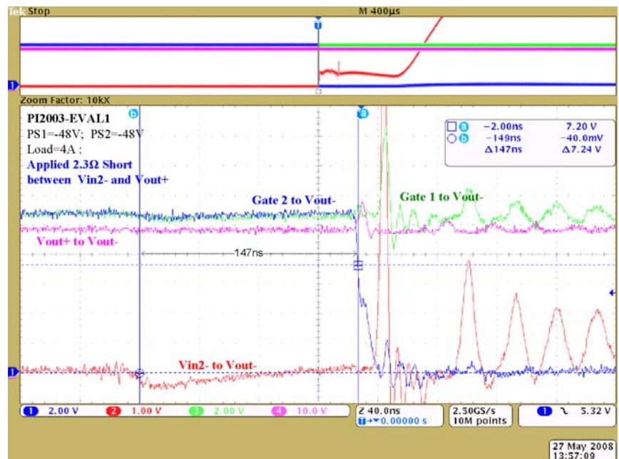
Figure 16: PI2003-EVAL1 performance under an input short
