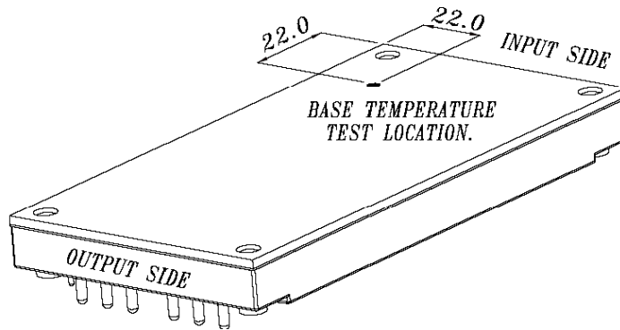
Fig. 4 Baseplate Temperature Measure Point.
