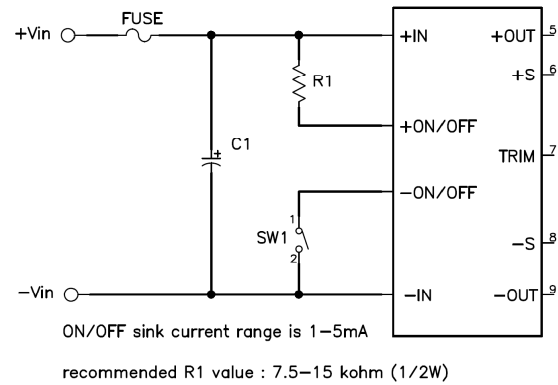
Fig. 3 ON/OFF Control Circuit
