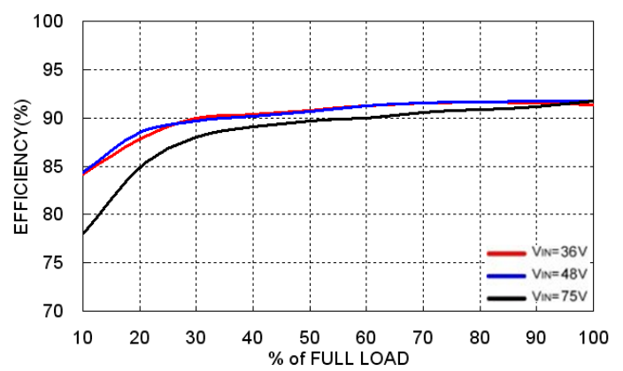
FED60-48S12 Efficiency VS Output Load
