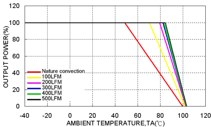
FED60-48S12 Derating Curve
