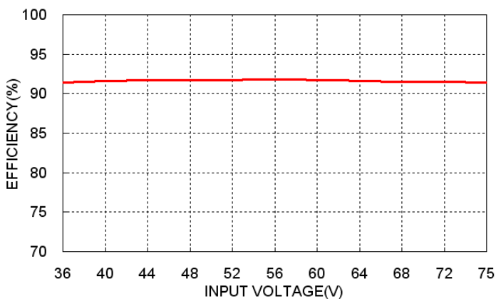
FED60-48S12 Efficiency VS Input Voltage
