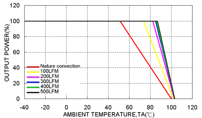
FED60-48S12 Derating Curve with Heat-sink
