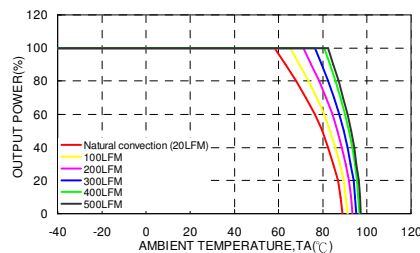
HAE75-48S05W Derating Curve (Note 2) With 0.24" Height Heat-sink
