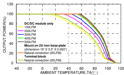
HAE200-48S05 Derating Curve (Note 3)
