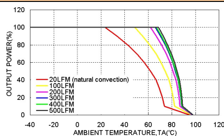
QAE100-48S05 Derating Curve With 0.24" Height Heat-sink
