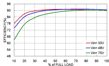
QAE100-48S05 Efficiency VS Output Load
